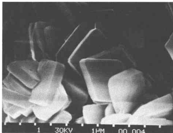
Fig. 4. Scanning Electron Microscope photograph of margaritasite crystals. The distance between tick marks is 1 \mu\text{m} .
