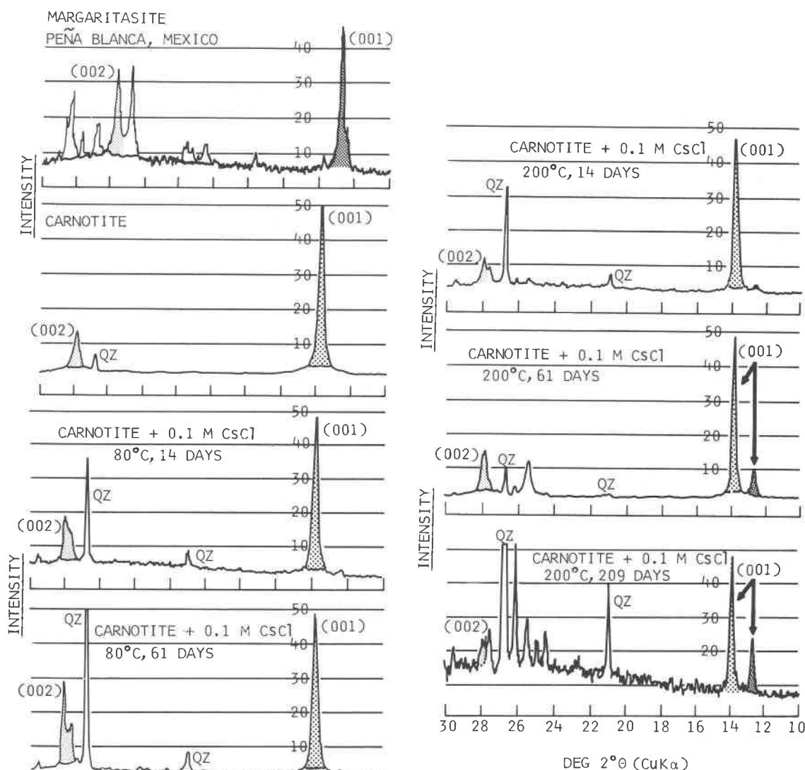
Fig. 6. X-ray powder diffraction patterns for margaritasite, Colorado Plateau carnotite and synthesized Cs-carnotite.
