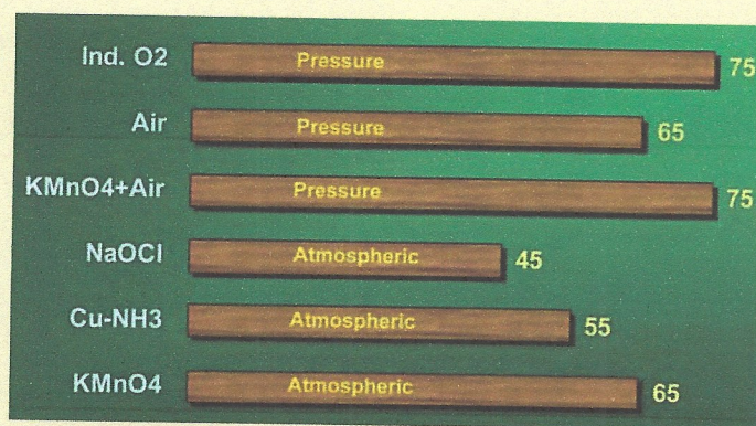
Fig. 3: Uranium leachability with various oxidants
