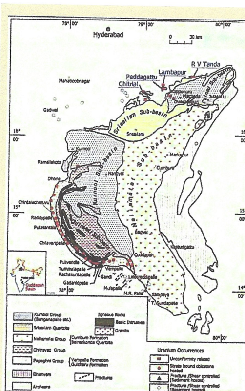
Fig. 1: Geological map of Kadapa basin showing uranium occurrences
