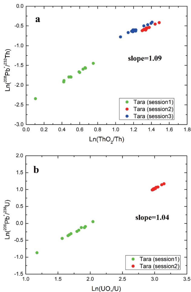
Fig. 2 Inter-elemental calibration diagrams of TARA allanites: (a) plot of secondary \ln(^{208}\text{Pb}^+ / ^{232}\text{Th}^+) versus \ln(\text{ThO}_2^+ / \text{Th}^+) ratios for TARA standard analyses; (b) plot of secondary \ln(^{206}\text{Pb}^+ / ^{238}\text{U}^+) versus \ln(\text{UO}_2^+ / \text{U}^+) ratios for TARA standard analyses.
