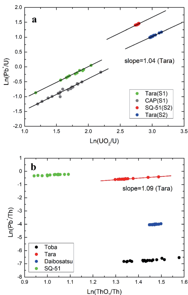
Fig. 6 Inter-elemental calibration diagrams. (a) Plot of \ln(^{206}\text{Pb}^*/^{238}\text{U}^+) versus \ln(\text{UO}_2^{+}/\text{U}^+) ratios for TARA standard analyses, where S1 and S2 represent different analyzing sessions; (b) plot of \ln(^{208}\text{Pb}^*/^{232}\text{Th}^+) versus \ln(\text{ThO}_2^{+}/\text{Th}^+) ratios for TARA standard analyses, where the \ln(^{208}\text{Pb}^*/^{232}\text{Th}^+) values of Toba measurements are corrected by the proportional relationship between TARA standard measurements in these two sessions.
