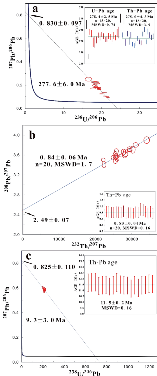
Fig. 4 Age results of allanite samples. (a) CAP measurements plotted in Tera–Wasserburg diagram with weighted average U–Pb and Th–Pb ages inserted; (b) TOBA Th–Pb isochron age with weighted average Th–Pb age inserted; (c) Daibosatsu measurements plotted in Tera–Wasserburg diagram with weighted average Th–Pb age inserted. Data point error bars and weighted average age uncertainties are at 2\sigma level.
