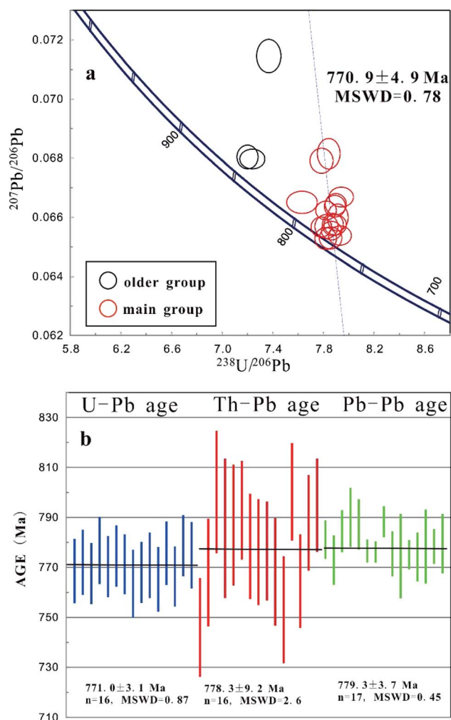
Fig. 5 Age results of SQ-51 allanites. (a) SQ-51 measurements plotted in Tera–Wasserburg diagram. (b) Weighted average U–Pb, Th–Pb and Pb–Pb ages for the main group. Data point error bars and weighted average age uncertainties are at 2σ level.
