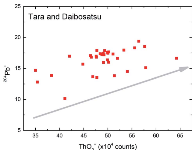
Fig. 3 Plot of \text{ThO}_2^+ versus {}^{204}\text{Pb}^+ indicating the interference of {}^{232}\text{Th}^{144}\text{Nd}^{16}\text{O}_2^{2+} on {}^{204}\text{Pb}^+ , the Tara and Daibosatsu measurements were conducted in a same session.
